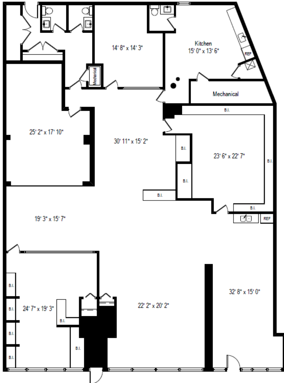
Floorplan
