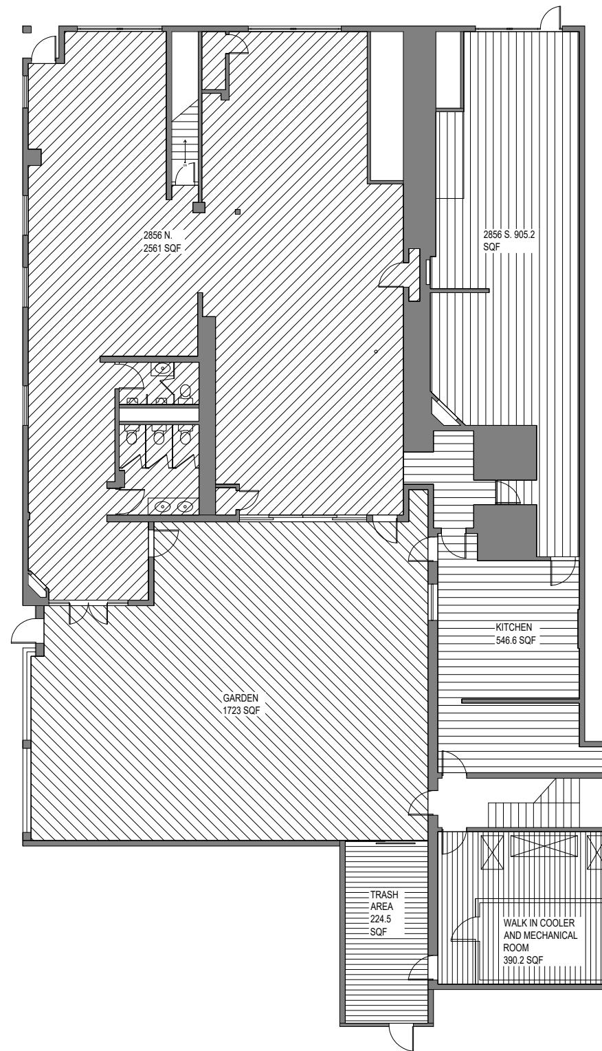
1ST FLOOR- 2856 N AND S UNITS
